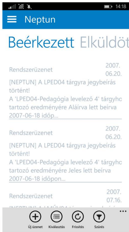
Windows Phone
